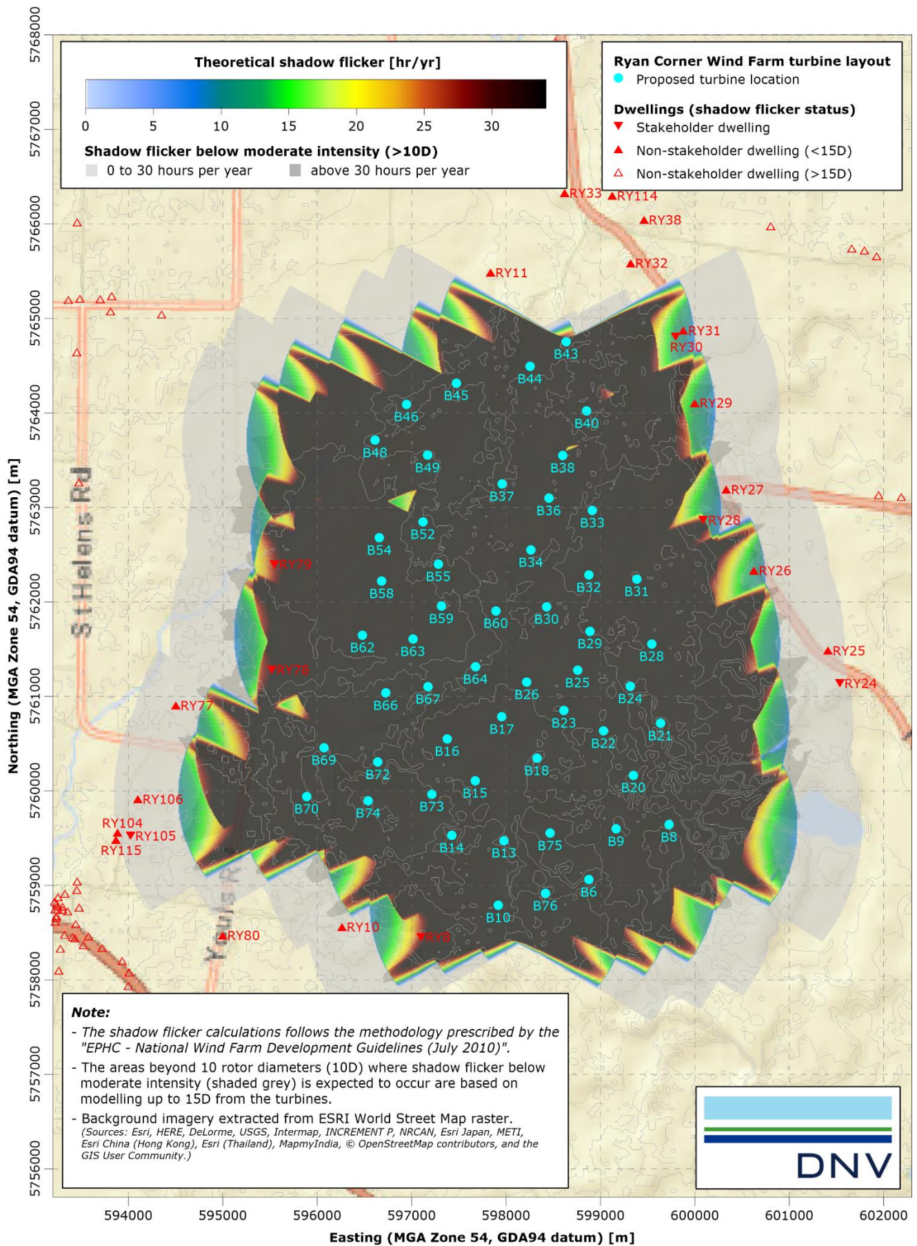
Figure 4 Theoretical annual shadow flicker duration map
