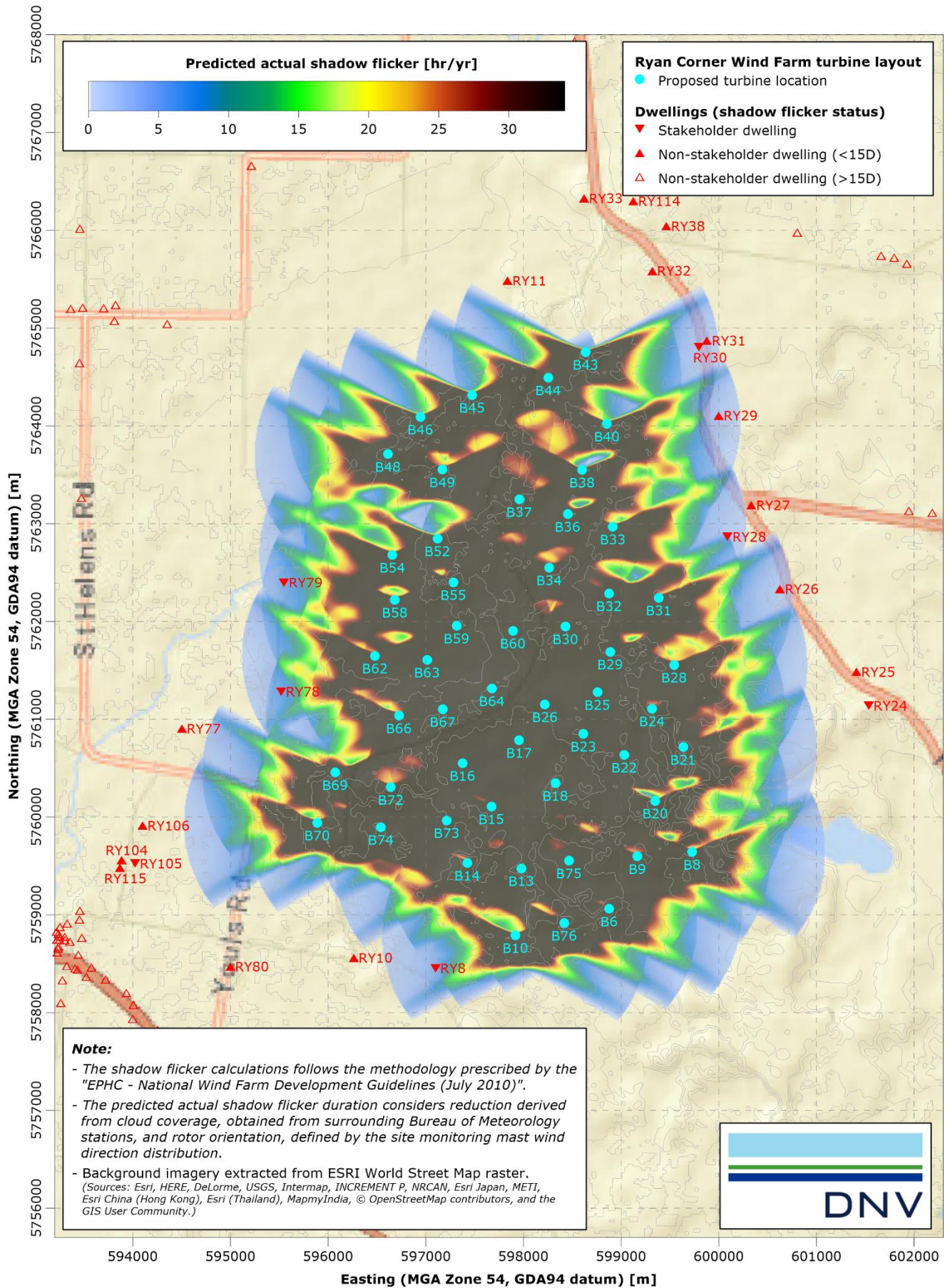
Figure 5 Predicted actual annual shadow flicker duration map
